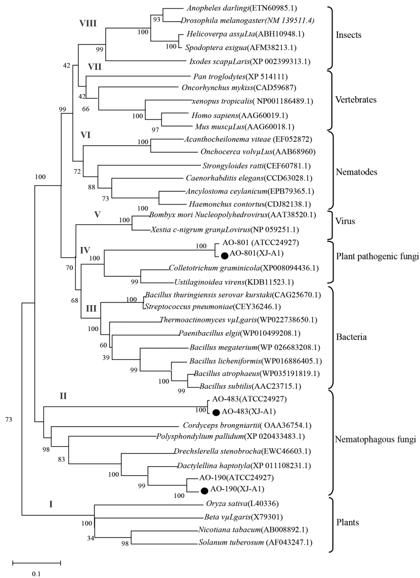
Supplementary Fig. S4. Phylogenetic analysis of chitinases genes among the different species. The chitinase genes AO-483 and AO-190 in the tree were from A. oligospora XJ-A1 strain.
