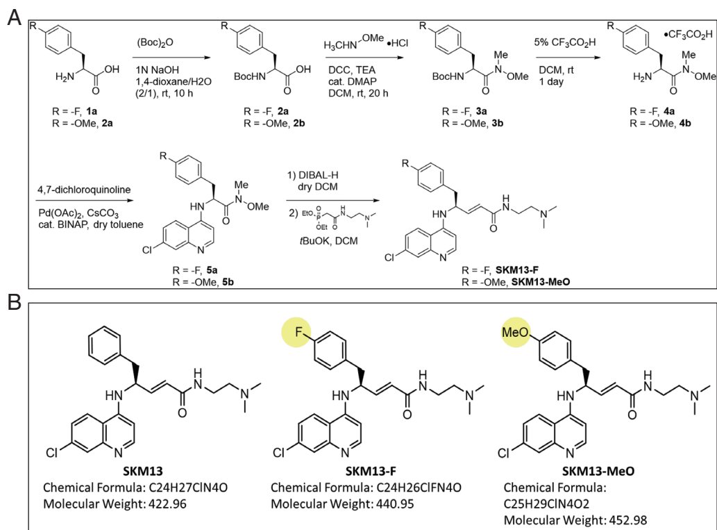
Supplementary Fig. S1. Synthesis of new anti-malarial drugs. (A) Scheme for Synthetic procedure for SKM13-F and SKM13-MeO through palladium-mediated N-C coupling. (B) Structure comparison between SKM13 and its novel derivatives (SKM13-F and SKM13-MeO).
